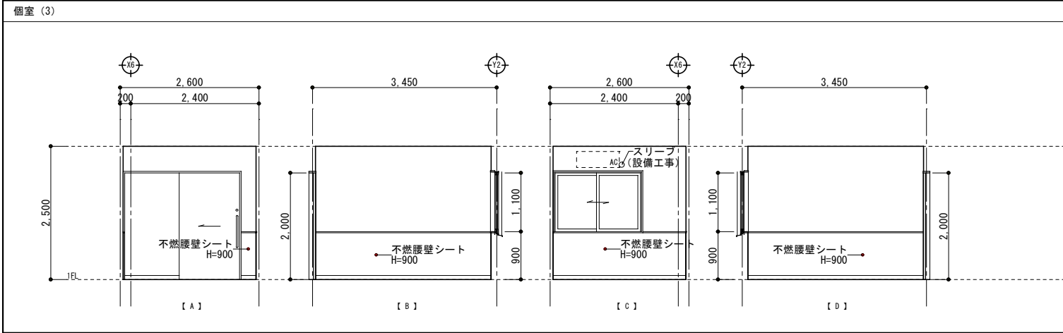
Figure 4 shows the elevation drawings of the four corners of the room, labeled [A], [B], [C], and [D]. The drawings illustrate the placement of non-combustible wall sheets (不燃腰壁シート) and the height of the sheets (H=900). The dimensions for each corner are as follows: [A]: Width 2,600, Height 2,500. The non-combustible wall sheet is located on the left wall. [B]: Width 3,450, Height 2,000. The non-combustible wall sheet is located on the bottom wall. [C]: Width 2,600, Height 2,500. The non-combustible wall sheet is located on the right wall. The AC unit (エアコン) is located on the top wall. [D]: Width 3,450, Height 2,000. The non-combustible wall sheet is located on the bottom wall.
